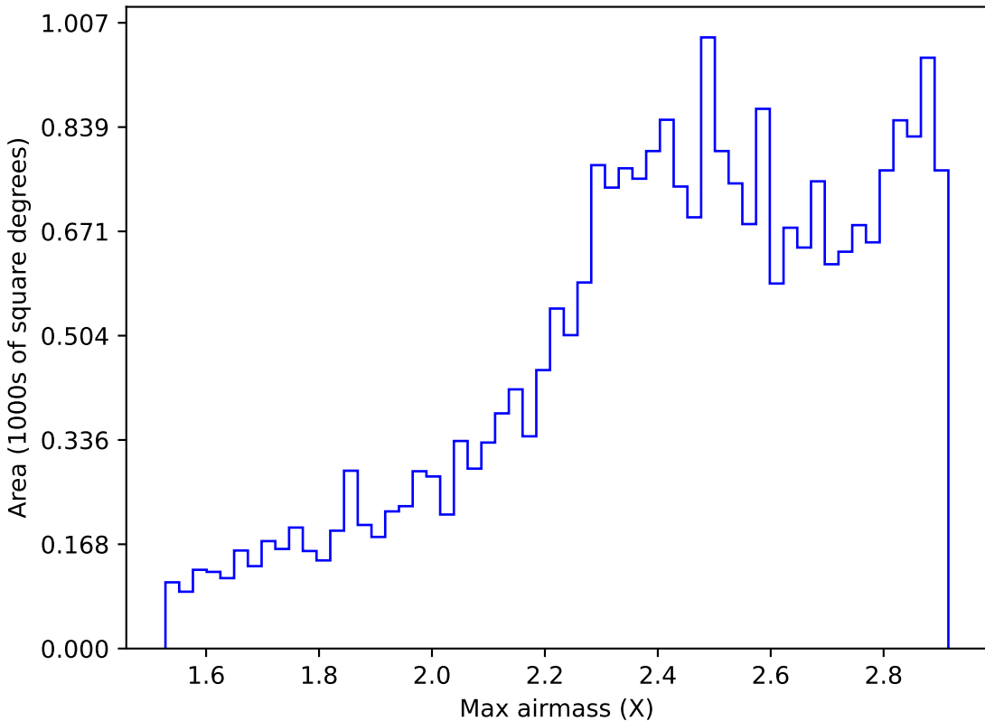
roman_v3.3_10yrs All sky i band: Max airmass
