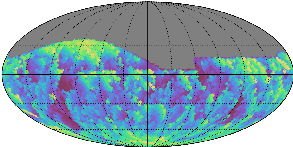
roman_v3.3_10yrs All sky g band: Max airmass
