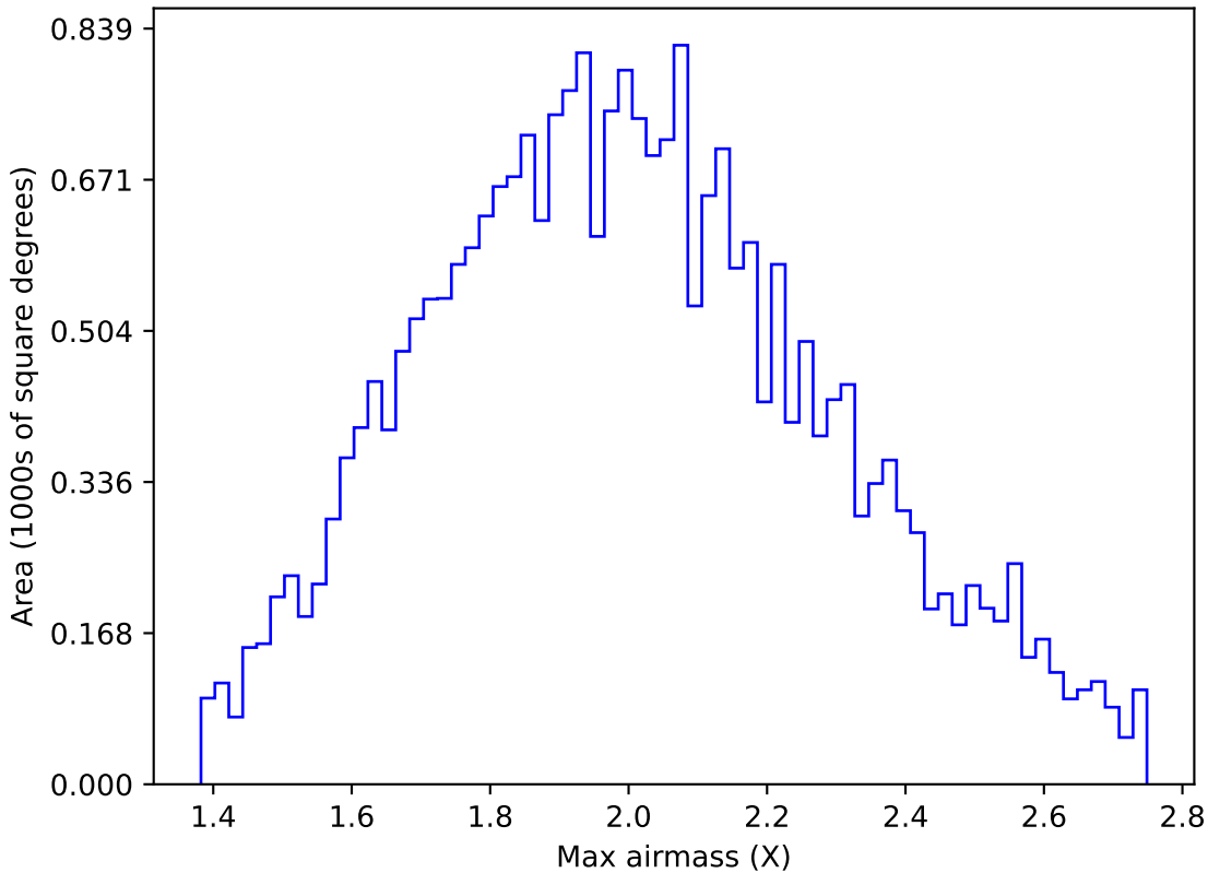
roman_v3.3_10yrs All sky g band: Max airmass
