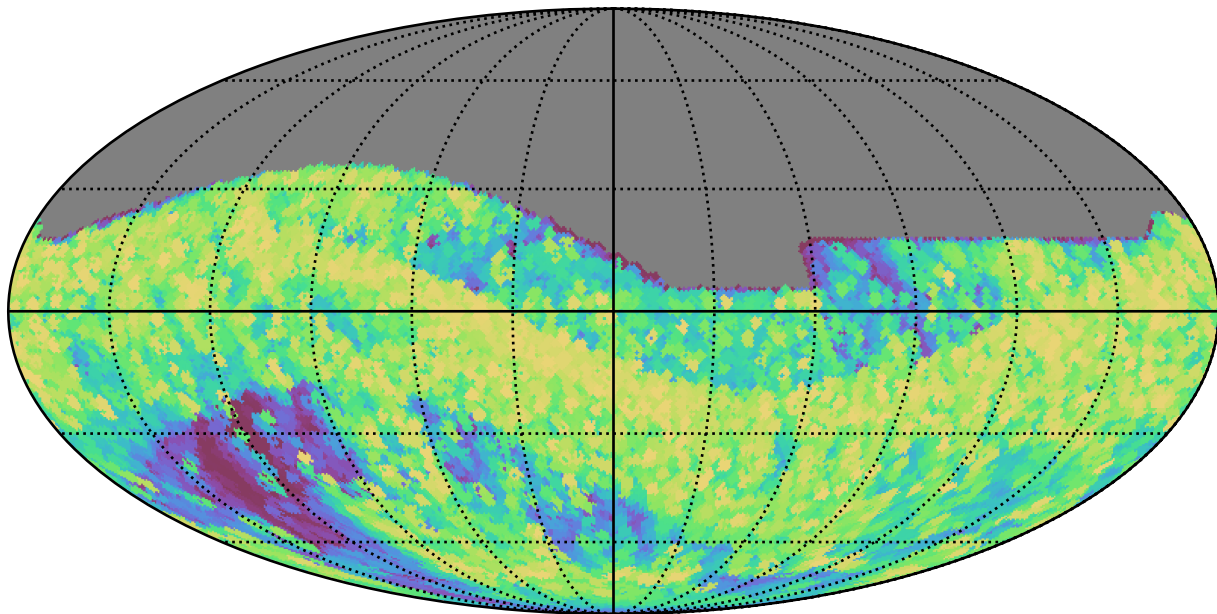
roman_v3.3_10yrs All sky all bands: Max airmass
