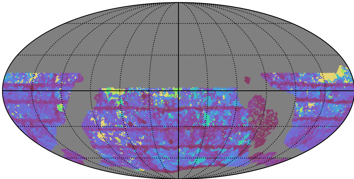
roman_v3.3_10yrs WFD z band: Max Inter-Night Gap
