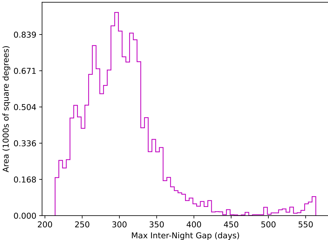
roman_v3.3_10yrs WFD z band: Max Inter-Night Gap
