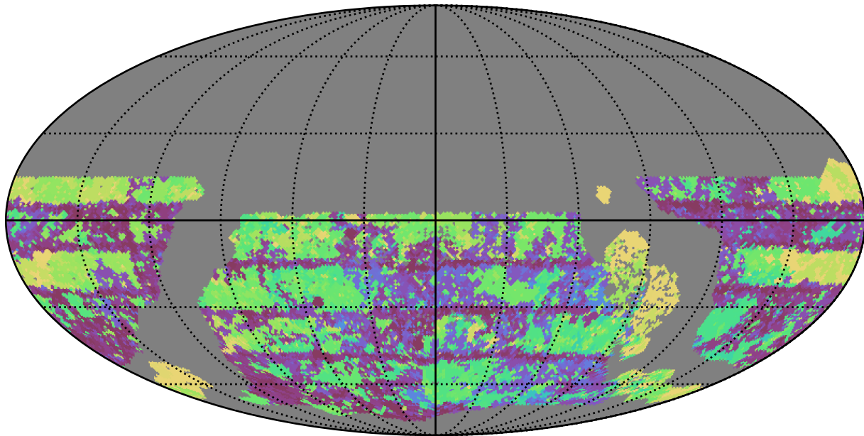
roman_v3.3_10yrs WFD u band: Max Inter-Night Gap
