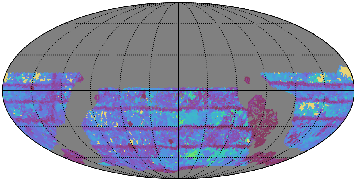
roman_v3.3_10yrs WFD r band: Max Inter-Night Gap
