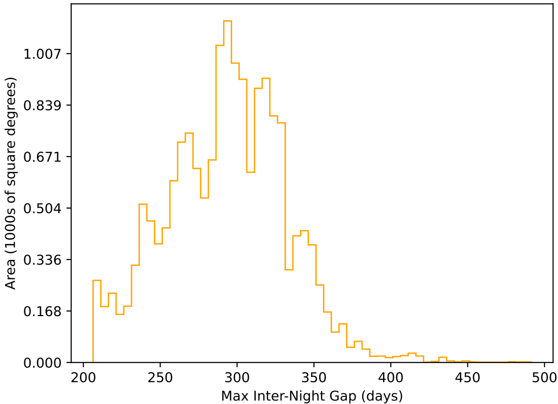
roman_v3.3_10yrs WFD r band: Max Inter-Night Gap
