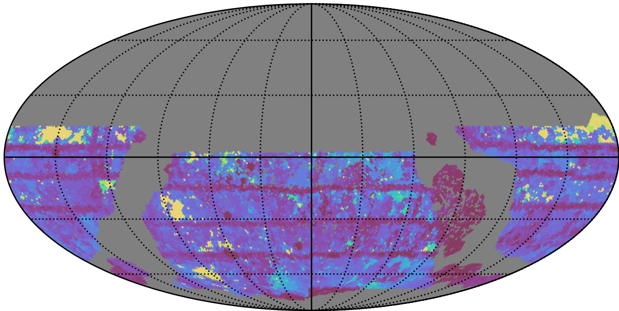
roman_v3.3_10yrs WFD i band: Max Inter-Night Gap
