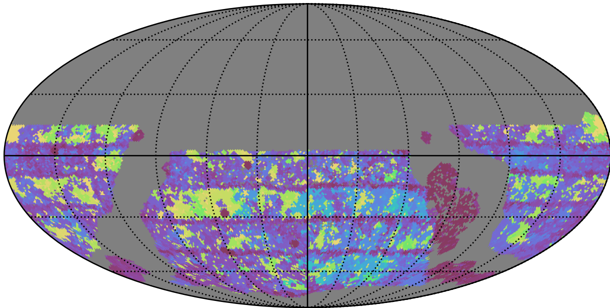
roman_v3.3_10yrs WFD g band: Max Inter-Night Gap
