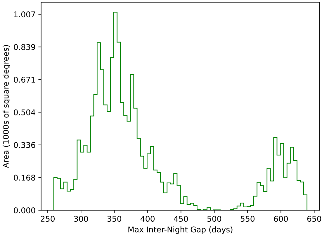
roman_v3.3_10yrs WFD g band: Max Inter-Night Gap
