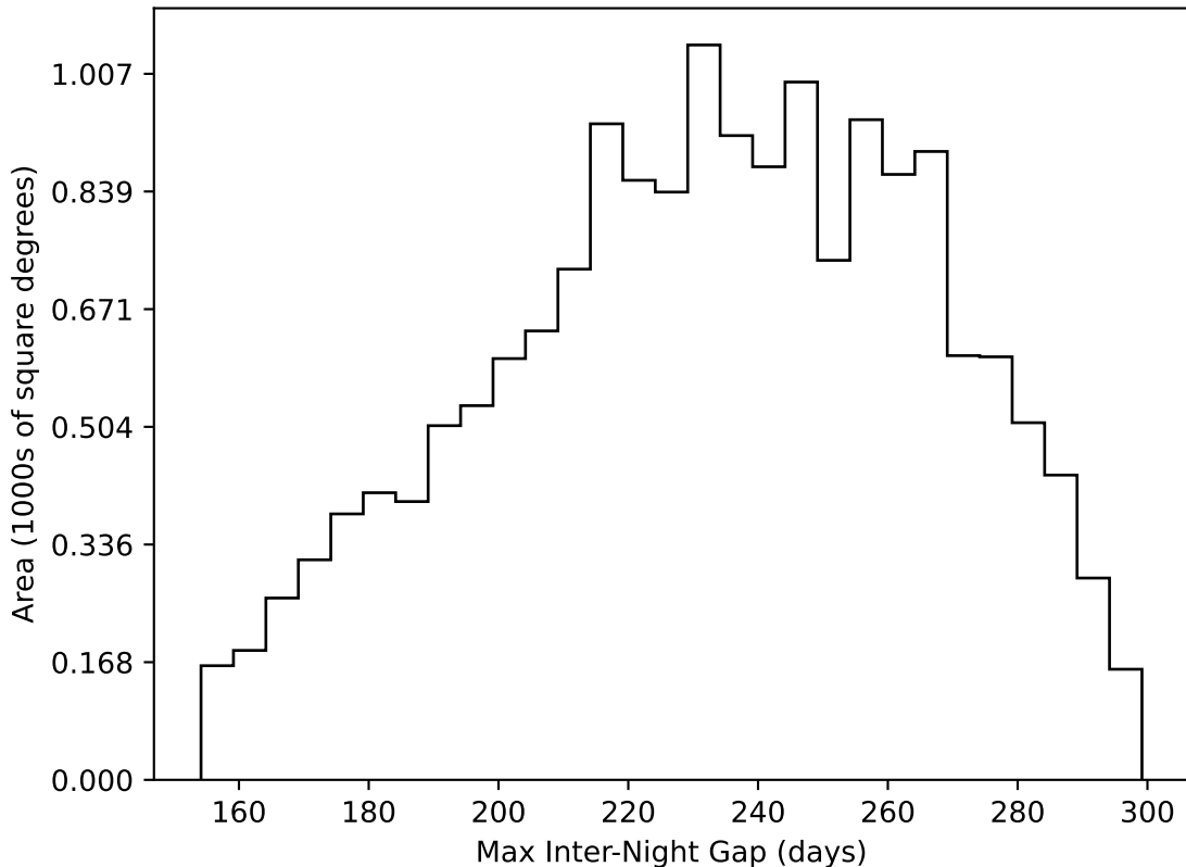
roman_v3.3_10yrs WFD all bands: Max Inter-Night Gap
