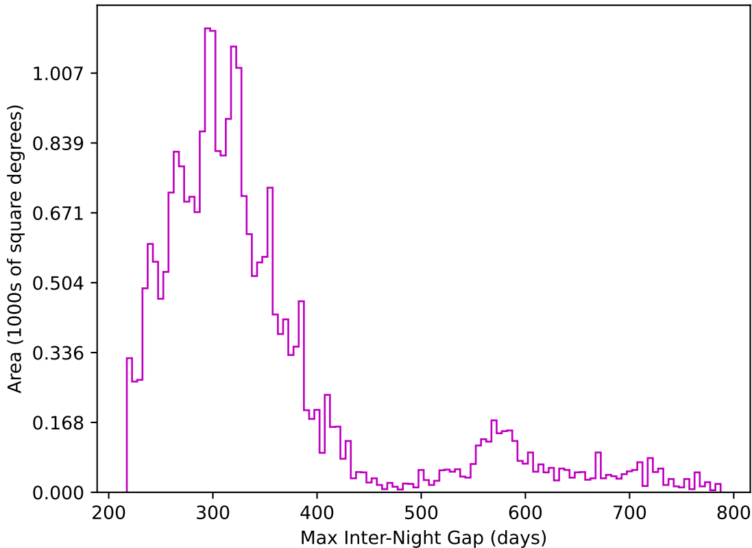
roman_v3.3_10yrs All sky z band: Max Inter-Night Gap
