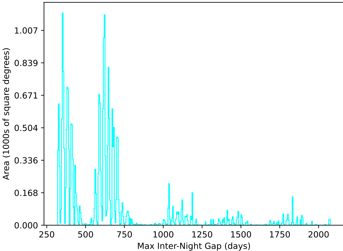
roman_v3.3_10yrs All sky u band: Max Inter-Night Gap
