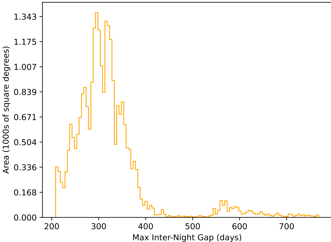
roman_v3.3_10yrs All sky r band: Max Inter-Night Gap
