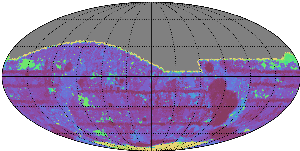
roman_v3.3_10yrs All sky i band: Max Inter-Night Gap
