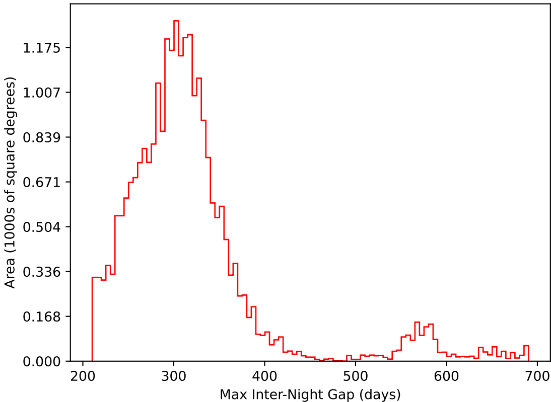
roman_v3.3_10yrs All sky i band: Max Inter-Night Gap
