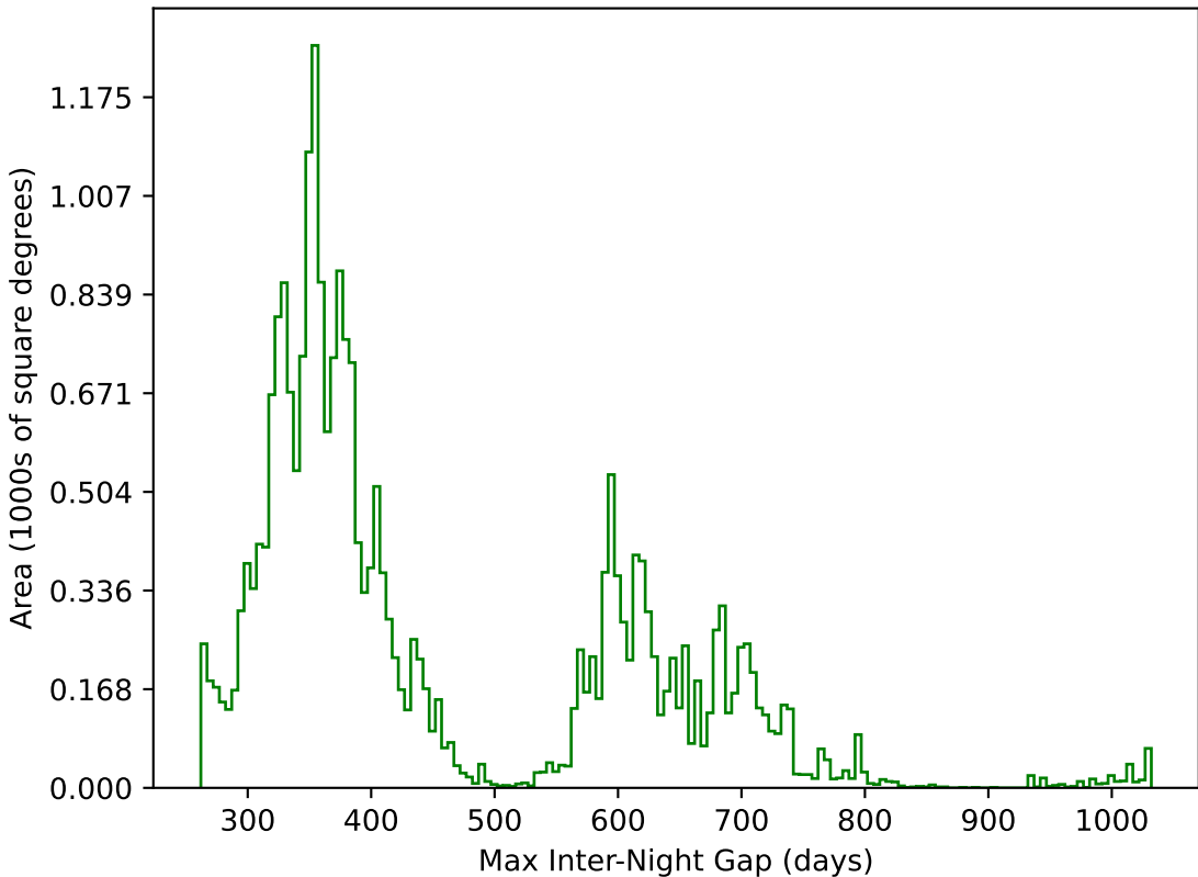
roman_v3.3_10yrs All sky g band: Max Inter-Night Gap
