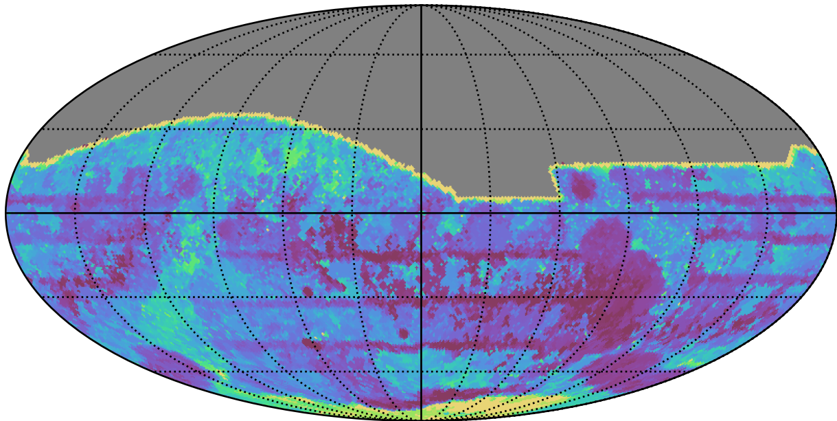
roman_v3.3_10yrs All sky all bands: Max Inter-Night Gap
