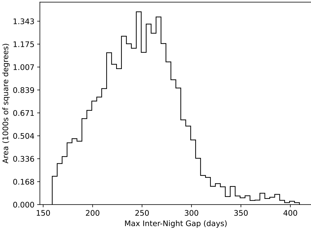
roman_v3.3_10yrs All sky all bands: Max Inter-Night Gap
