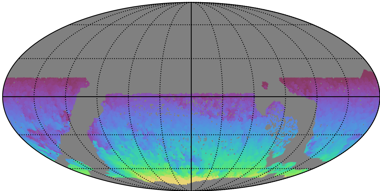
roman_v3.3_10yrs WFD all bands: Max HA
