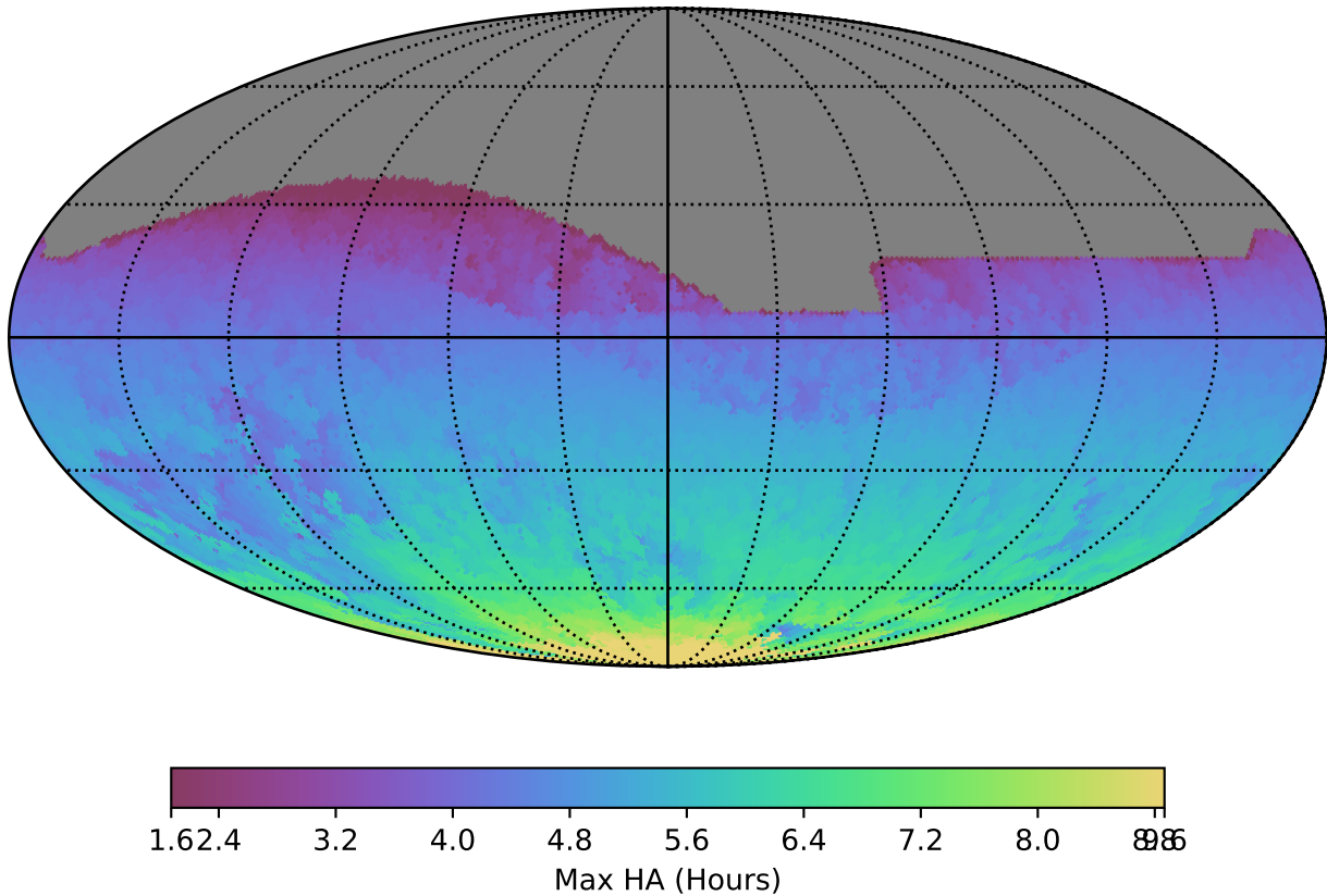
roman_v3.3_10yrs All sky all bands: Max HA
