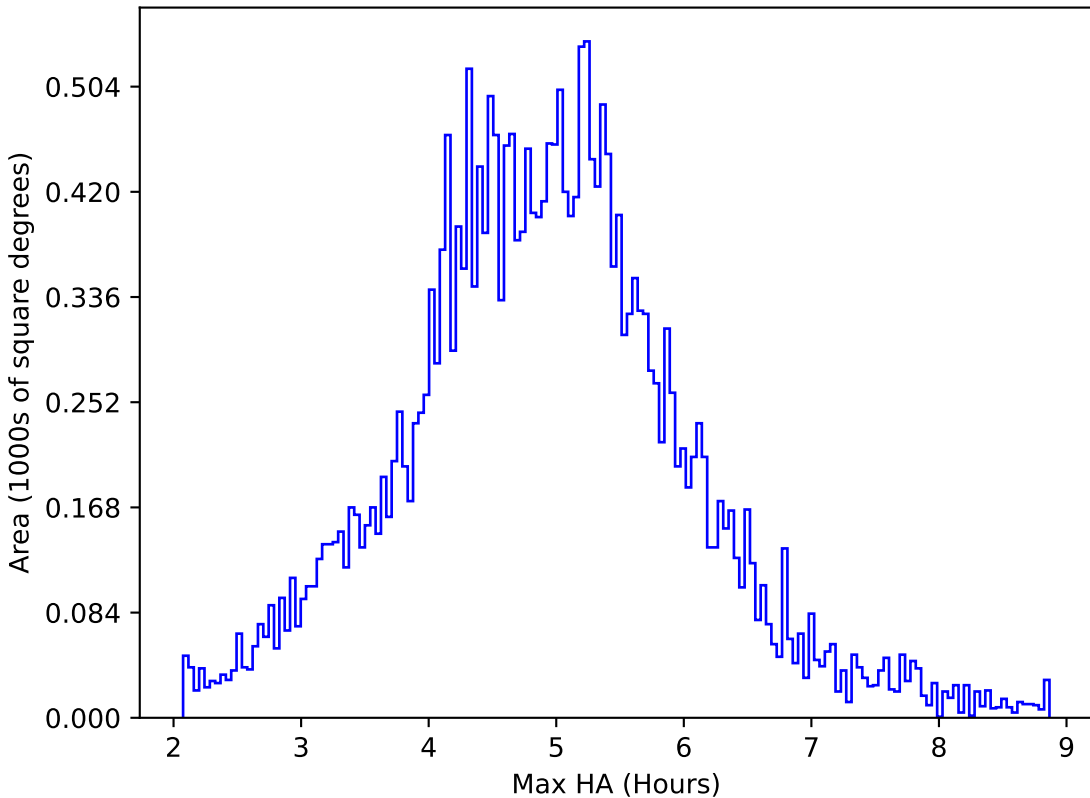
roman_v3.3_10yrs All sky all bands: Max HA
