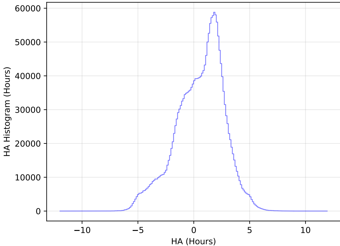
roman_v3.3_10yrs WFD all bands: HA Histogram
