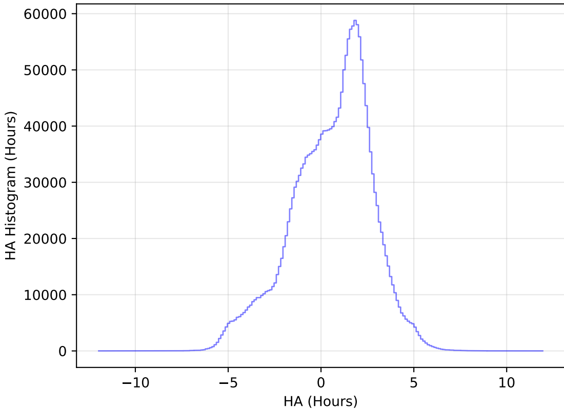
roman_v3.3_10yrs All sky all bands: HA Histogram
