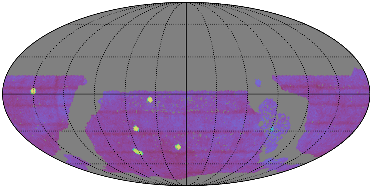
roman_v3.3_10yrs gri WFD: Fraction of visits with a revisit < 60 min
