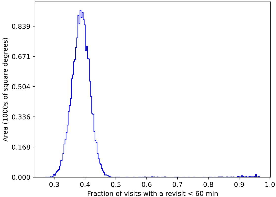
roman_v3.3_10yrs gri WFD: Fraction of visits with a revisit < 60 min
