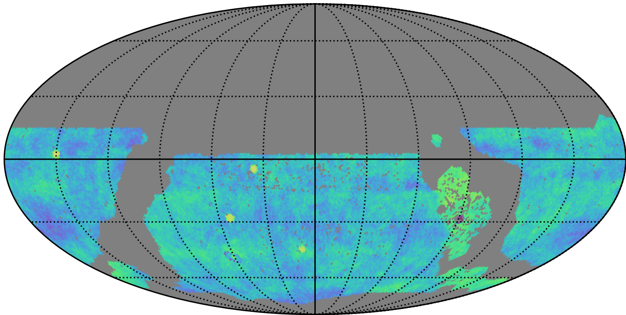
roman_v3.3_10yrs gri WFD: Fraction of visits in pairs (20-90 min)
