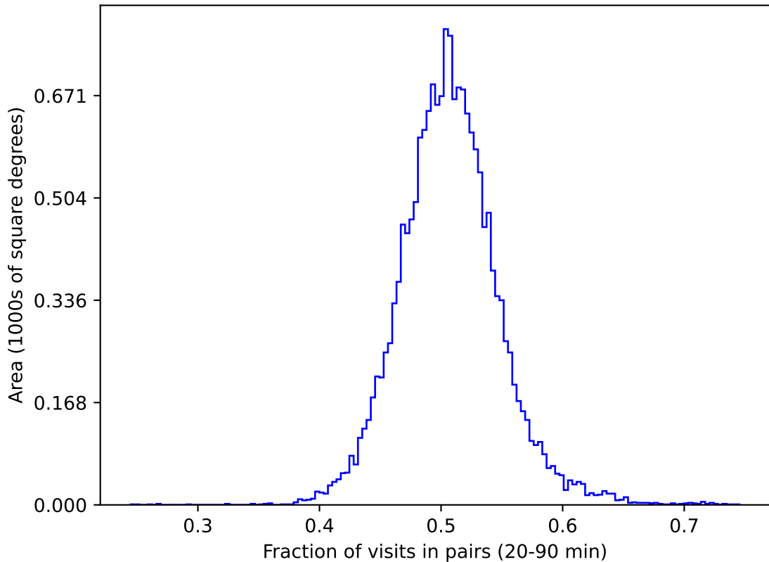
roman_v3.3_10yrs gri WFD: Fraction of visits in pairs (20-90 min)
