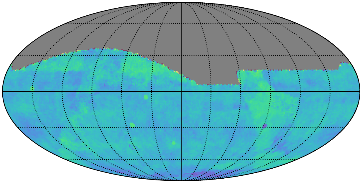
roman_v3.3_10yrs gri All sky: Fraction of visits in pairs (20-90 min)
