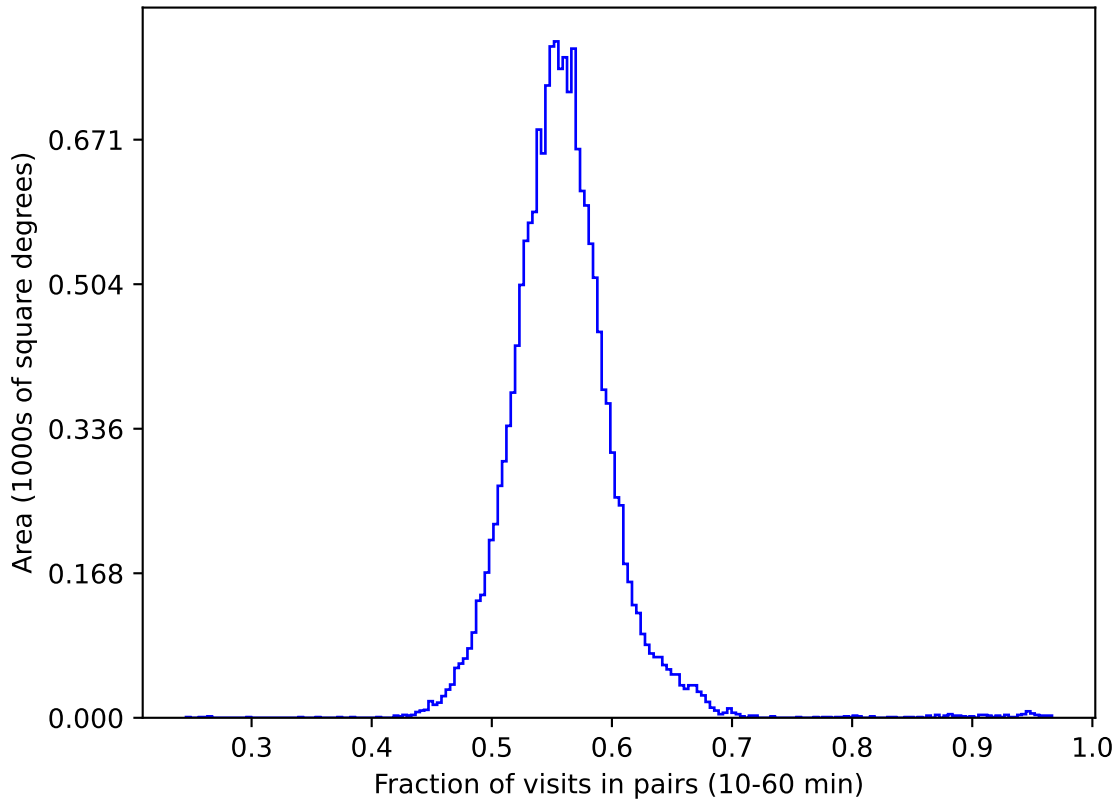
roman_v3.3_10yrs gri WFD: Fraction of visits in pairs (10-60 min)
