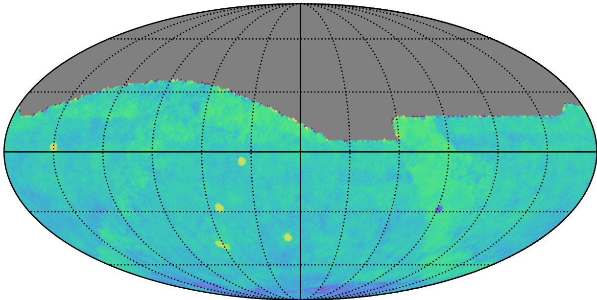
roman_v3.3_10yrs gri All sky: Fraction of visits in pairs (10-60 min)
