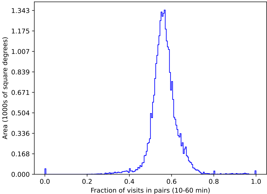
roman_v3.3_10yrs gri All sky: Fraction of visits in pairs (10-60 min)
