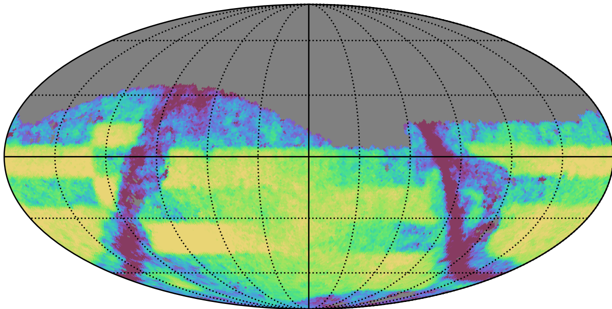
roman_v3.3_10yrs Yr 3-4 z band: Exgal_CoaddM5
