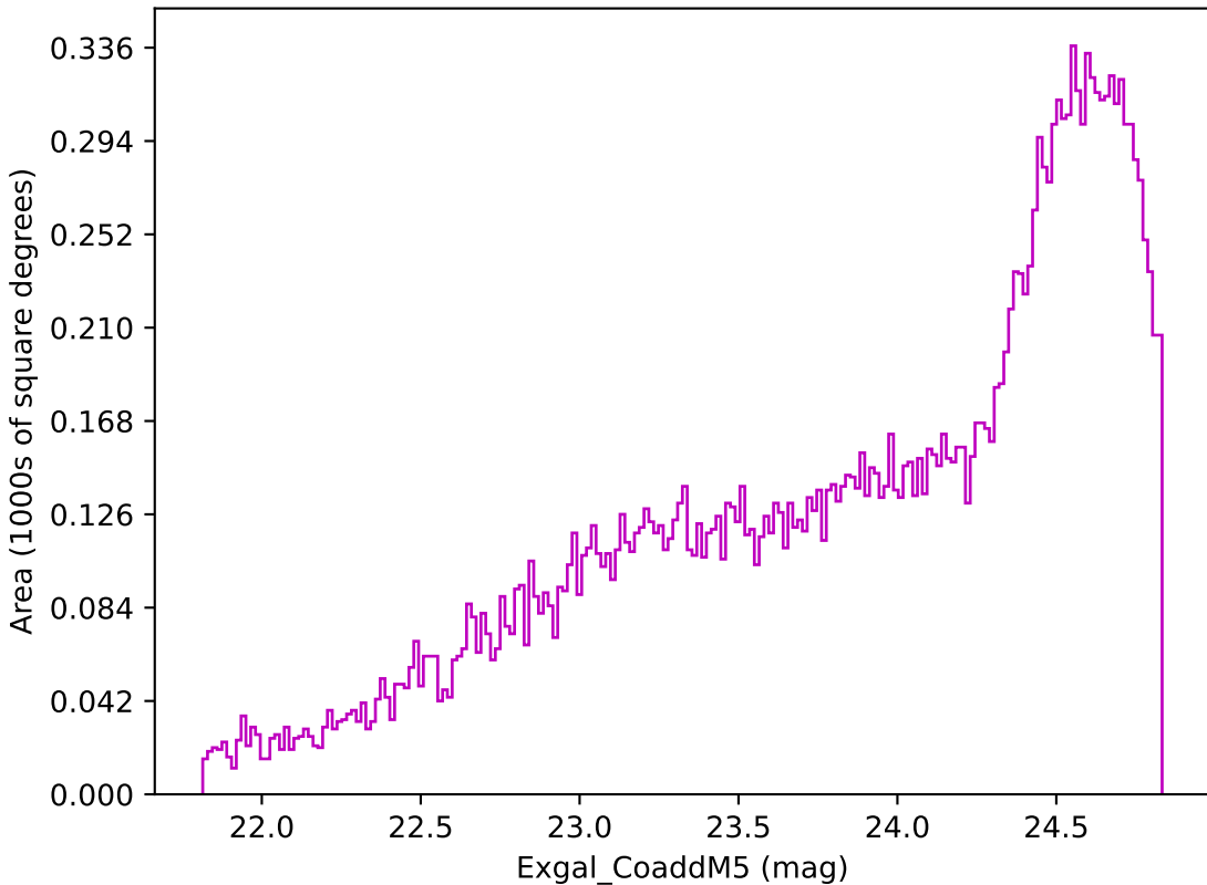
roman_v3.3_10yrs Yr 3-4 z band: Exgal_CoaddM5
