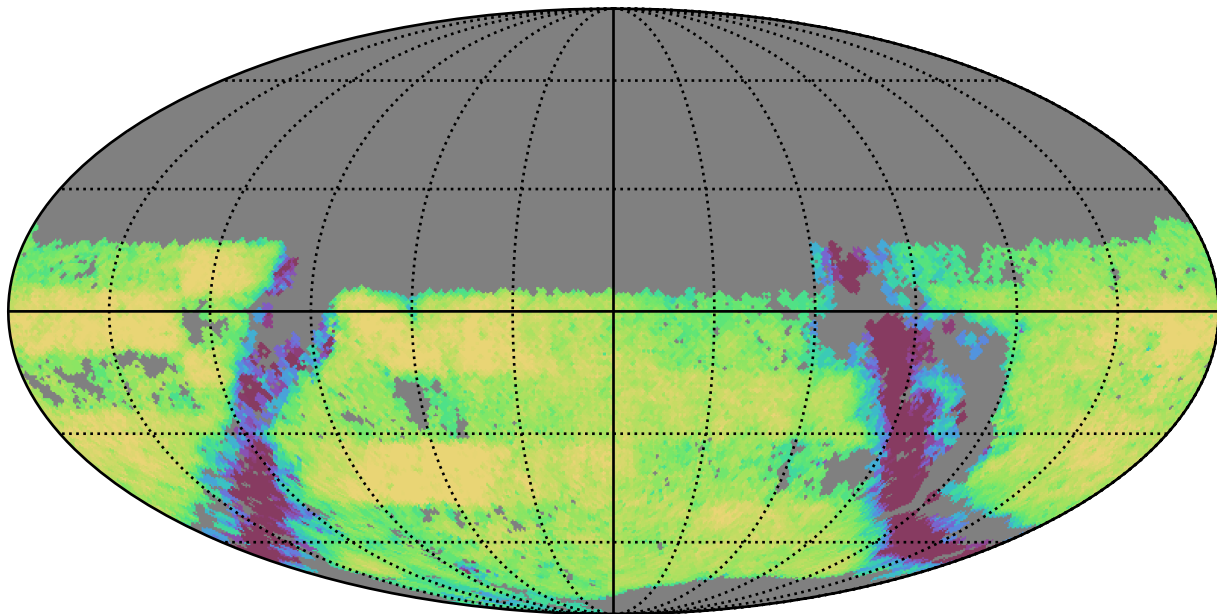
roman_v3.3_10yrs Yr 3-4 u band: Exgal_CoaddM5
