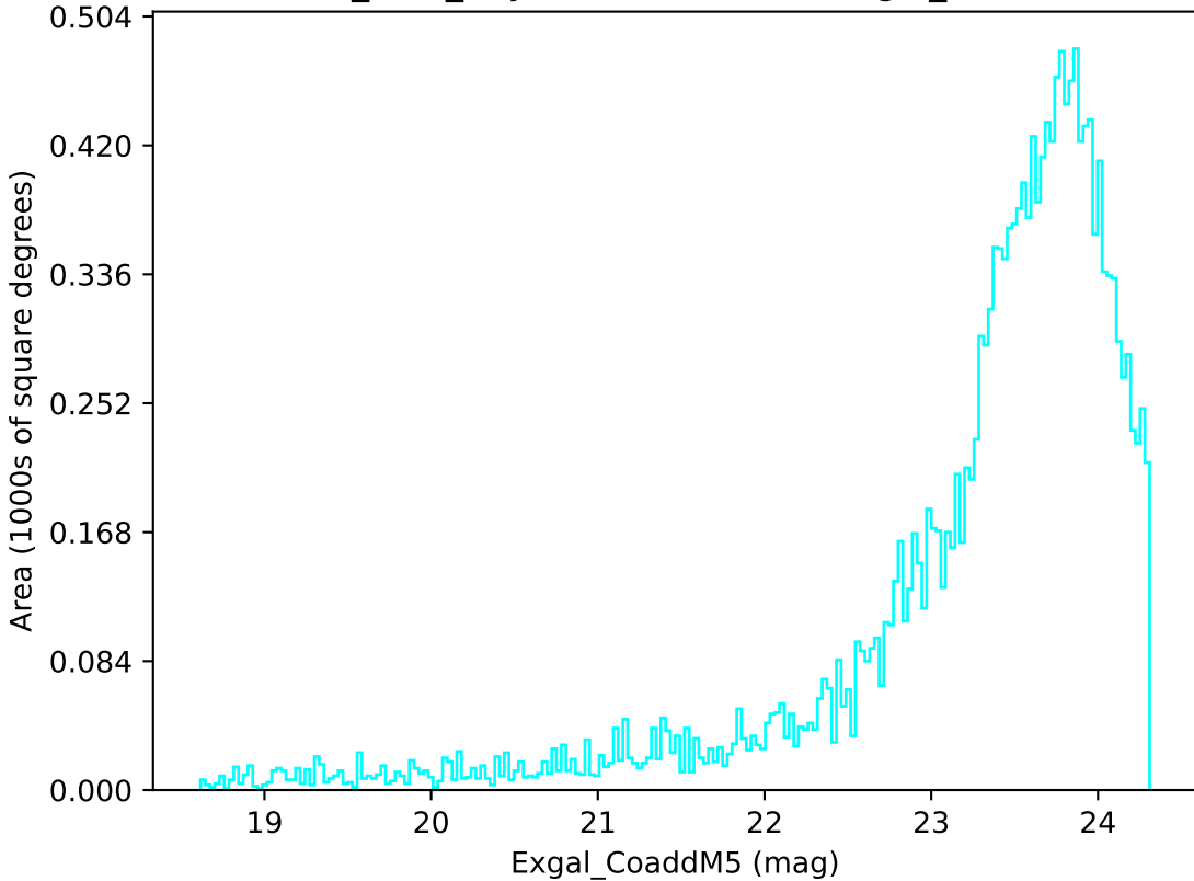
roman_v3.3_10yrs Yr 3-4 u band: Exgal_CoaddM5
