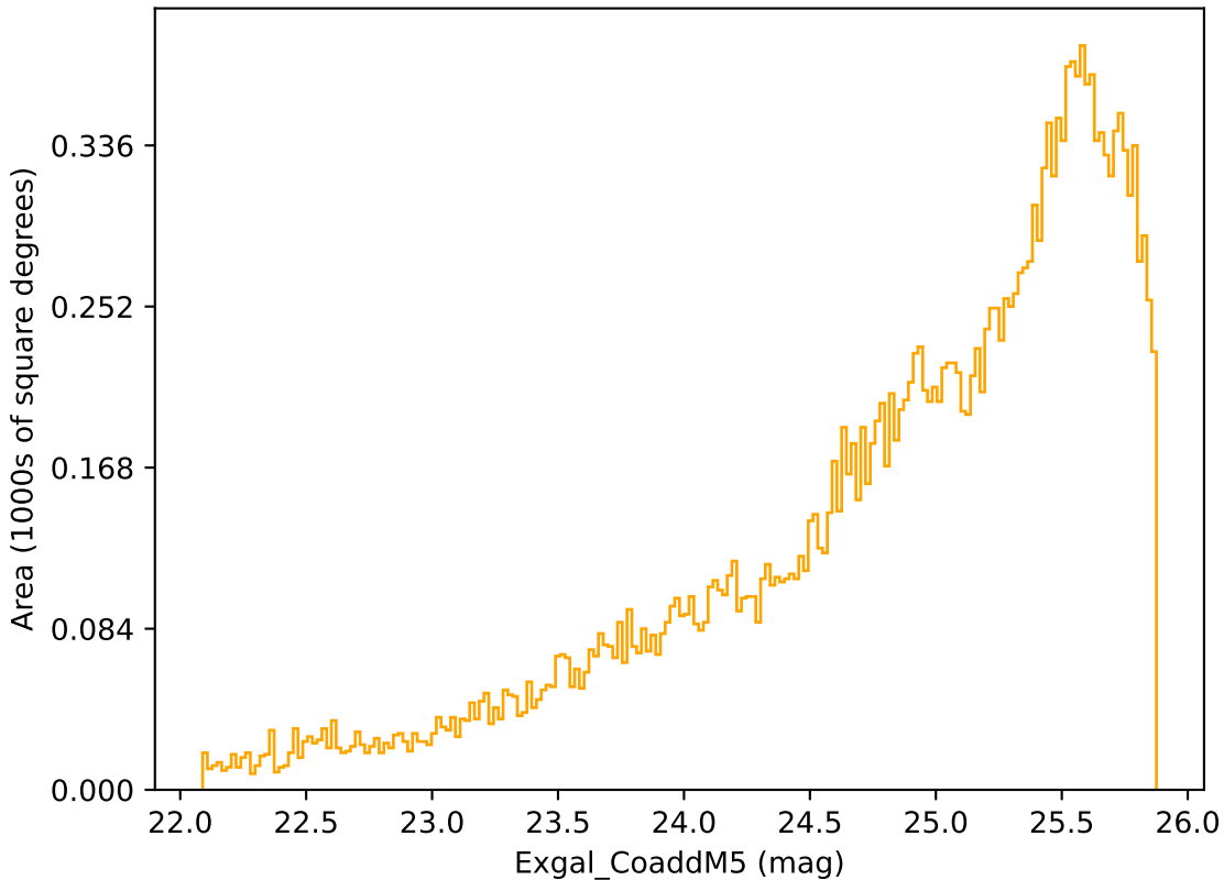
roman_v3.3_10yrs Yr 3-4 r band: Exgal_CoaddM5
