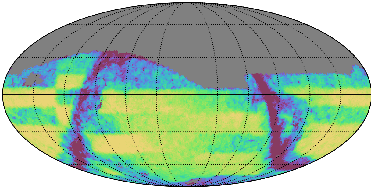
roman_v3.3_10yrs Yr 3-4 i band: Exgal_CoaddM5
