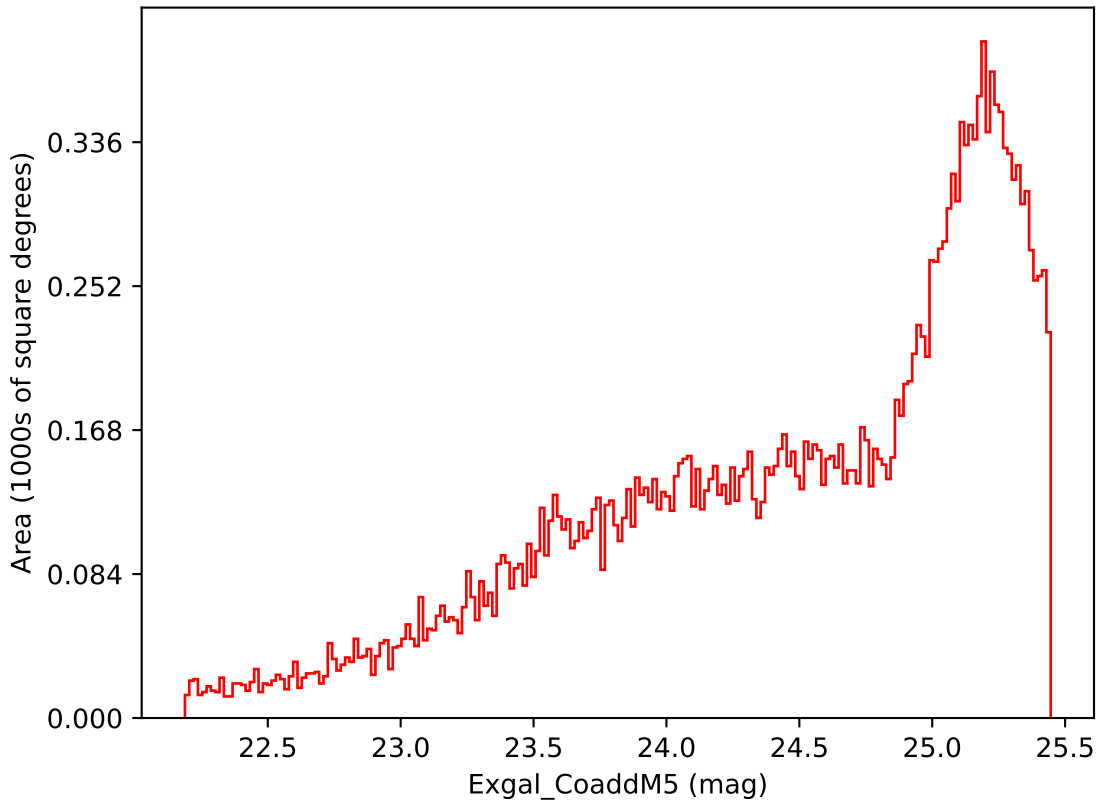
roman_v3.3_10yrs Yr 3-4 i band: Exgal_CoaddM5
