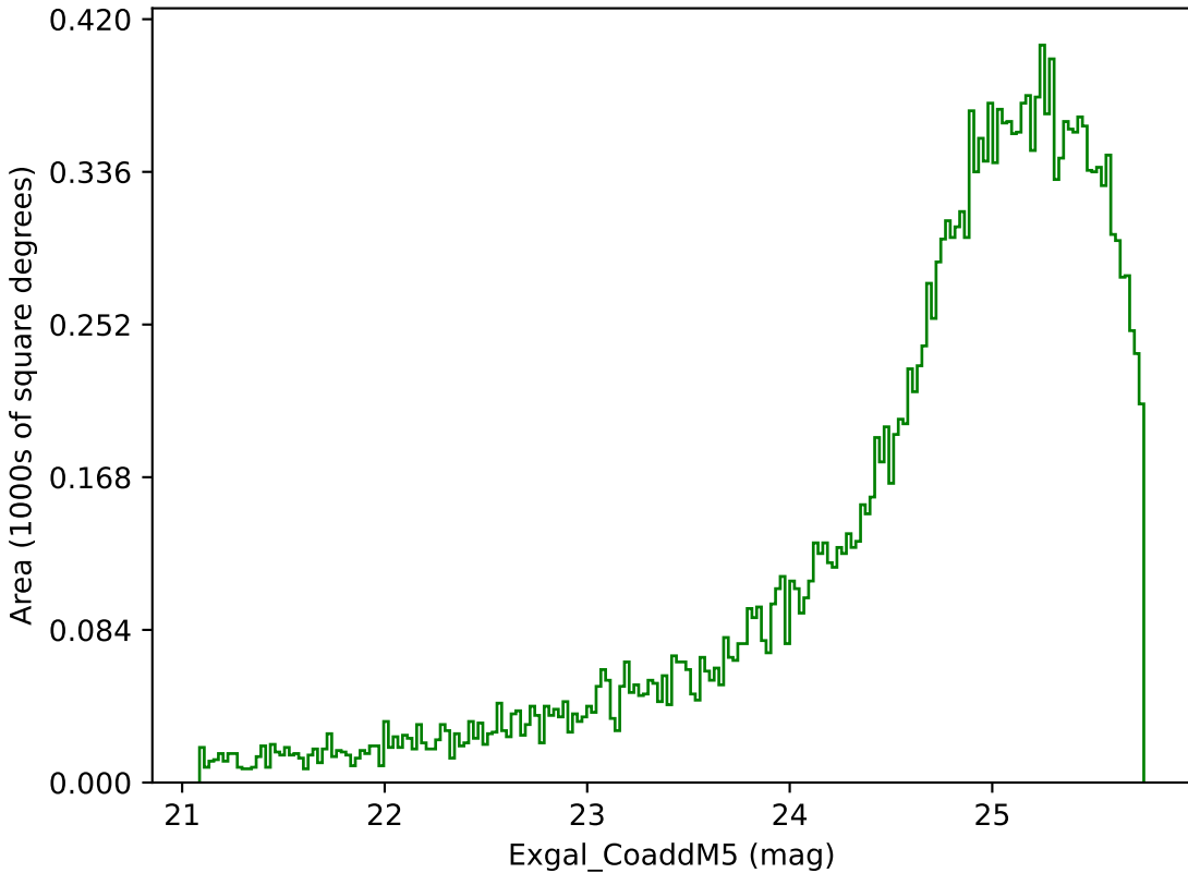
roman_v3.3_10yrs Yr 3-4 g band: Exgal_CoaddM5
