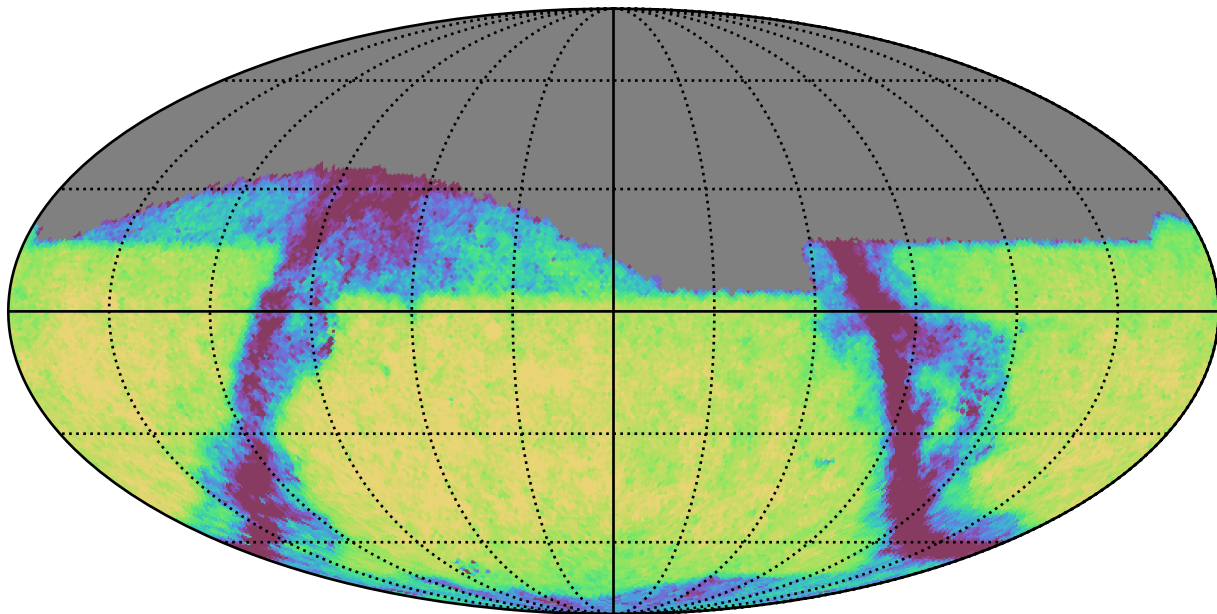
roman_v3.3_10yrs Yr 1 z band: Exgal_CoaddM5
