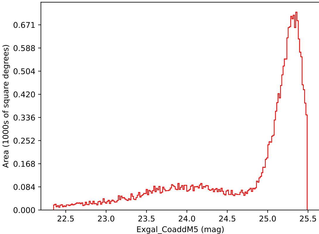
roman_v3.3_10yrs Yr 1 i band: Exgal_CoaddM5
