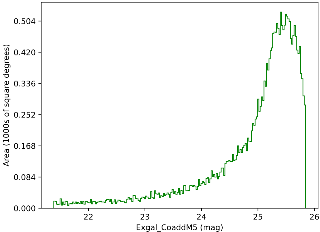
roman_v3.3_10yrs Yr 1 g band: Exgal_CoaddM5
