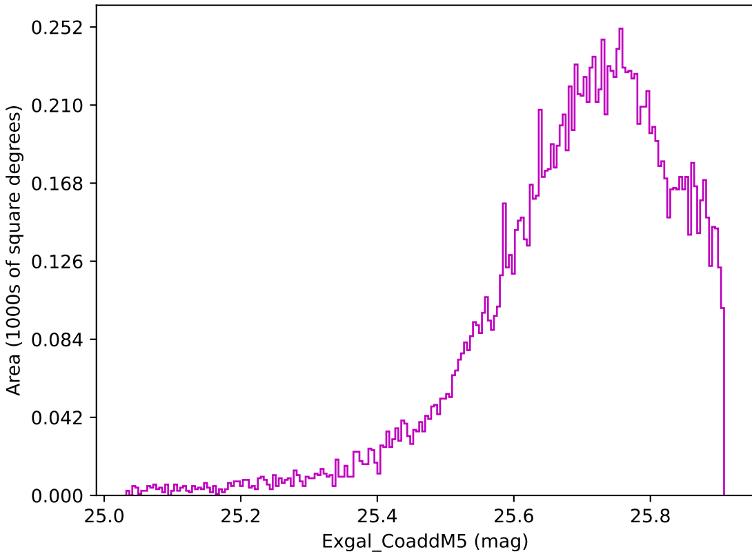
roman_v3.3_10yrs WFD z band: Exgal_CoaddM5
