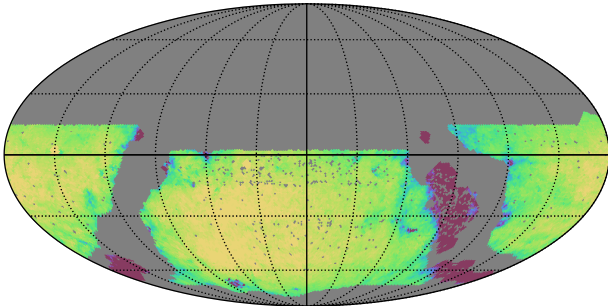
roman_v3.3_10yrs WFD u band: Exgal_CoaddM5
