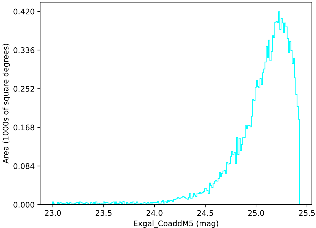
roman_v3.3_10yrs WFD u band: Exgal_CoaddM5
