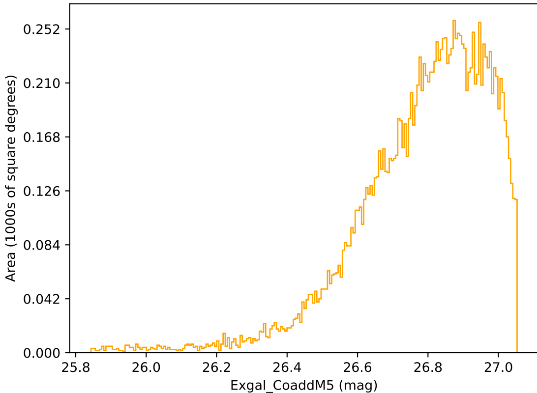
roman_v3.3_10yrs WFD r band: Exgal_CoaddM5
