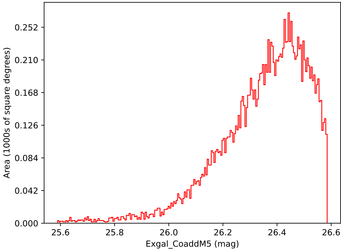
roman_v3.3_10yrs WFD i band: Exgal_CoaddM5
